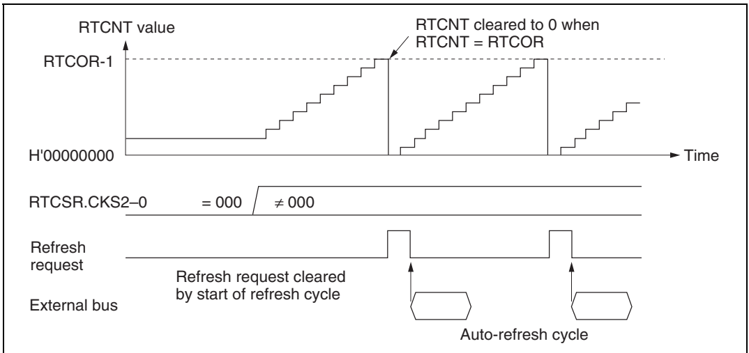
Figure 13.35 Auto-Refresh Operation
