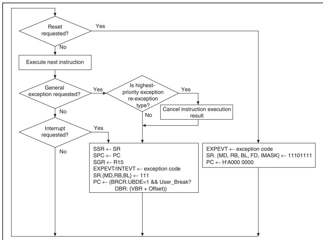
Figure 5.2 Instruction Execution and Exception Handling
