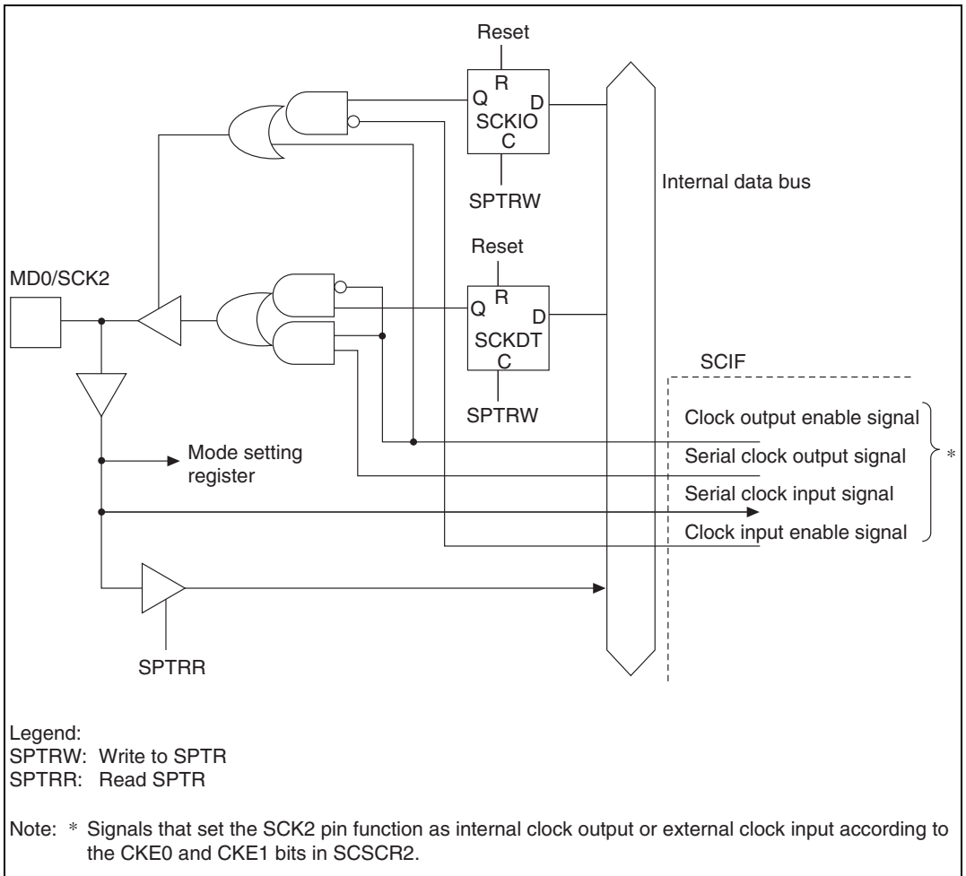
Figure 18.8 MD0/SCK2 Pin
