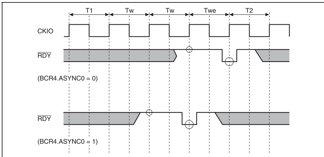
Figure 13.4 Example of \overline{\text{RDY}} Sampling Timing at which BCR4 Is Set (Two Wait Cycles Are Inserted by WCR2)
