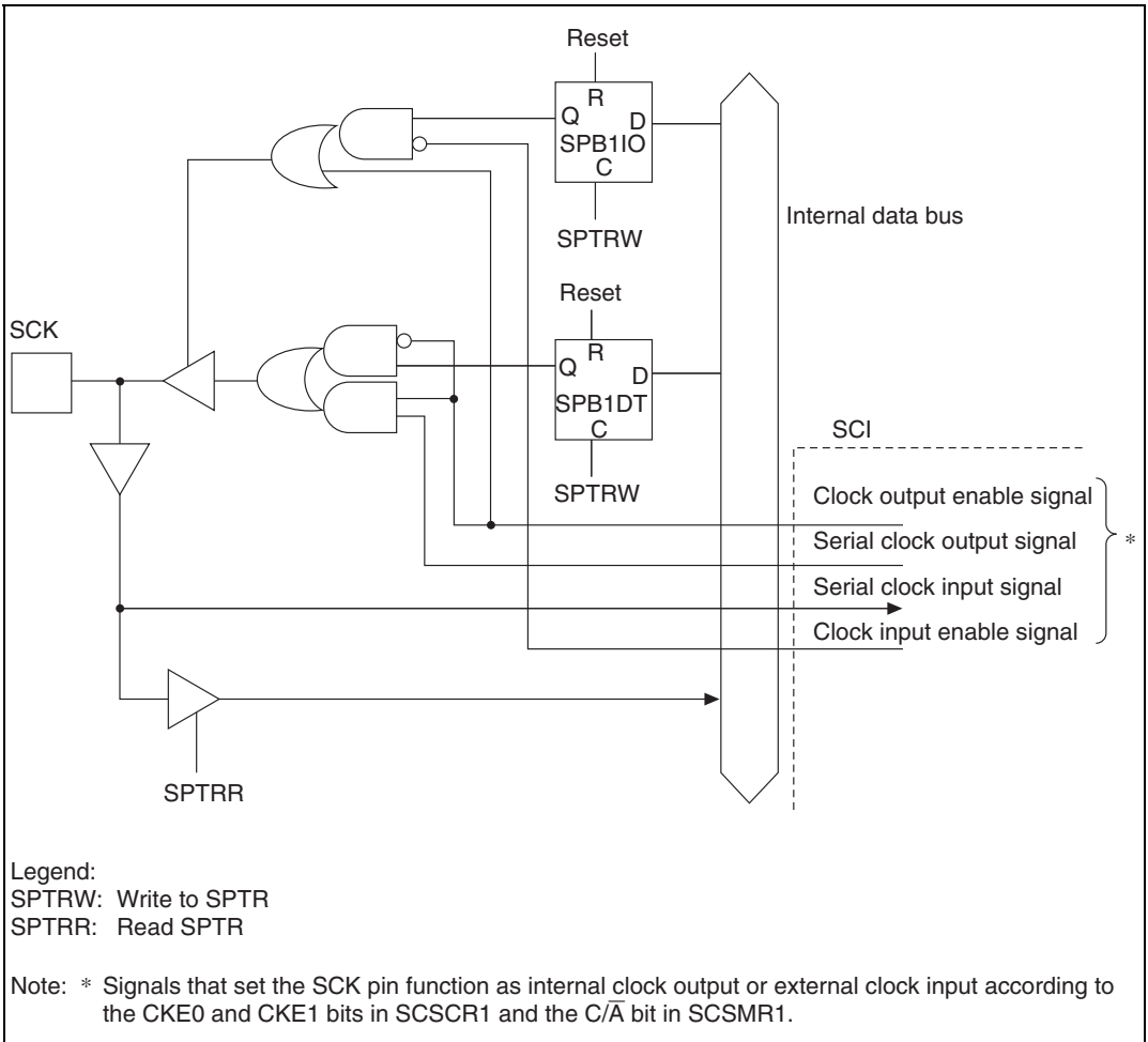
Figure 18.3 SCK Pin
